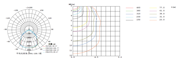
Light Distribution Curve
